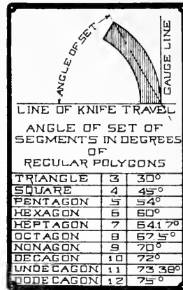
FIG. 212. TABLE FOR SEGMENTAL WORK ON TRIMMER.
